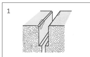
1 Milled joint in concrete, with broken-away area repaired
