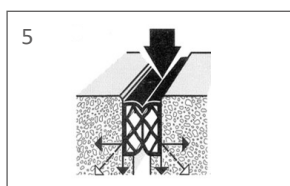
5 Absorption and distribution of vertical loads
