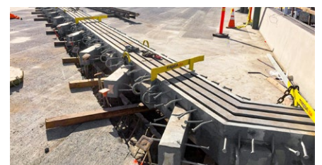
The delivered modular joint during installation
