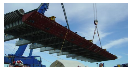
Installation of LR17 expansion joint featuring "Fuse-Box" seismic protection
