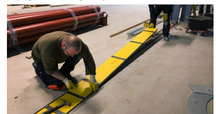
Laying and docking of a joint section
