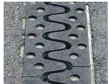
mageba RSFD cantilever finger joint with ROBO®GRIP
